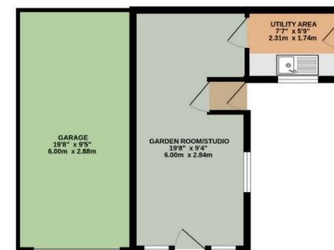
OUTBUILDING 229 sq.ft. (21.3 sq.m.) approx.
